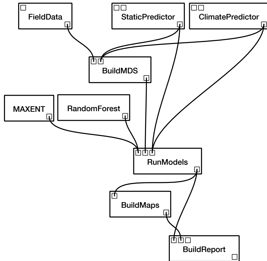
Figure 4.3: A representative workflow from a collection of workflows used for habitat modeling.
