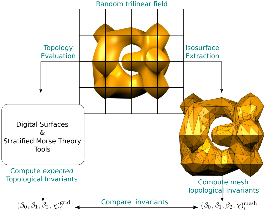
Figure 3.1. Overview of our topology verification pipeline. First step, we generate a random trilinear field and extract a random isosurface using the implementation under verification. We then compute the expected topological invariants from the trilinear field and compare them against the invariants obtained from the mesh.
