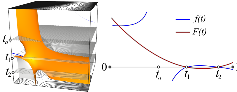
Figure 4.5. Counterexample to Chernyaev’s core disambiguation algorithm. The MC33 algorithm incorrectly interprets case 13.5.2 as 13.5.1. The left image shows the zero-level set for case 13.5.2 and cutting-planes at heights t_1 , t_2 , and t_a , which correspond to both roots of F(t) and the asymptote of f(x_c(t)) , respectively. The blue ribbon shows the path of the face saddle x_c(t) . The right image shows the changes in f(x_c(t)) and F(t) . According to the three criteria of the MC33 algorithm described in Section 4.2, the upward-facing red parabola defines the absence of a tunnel (condition (i)), which is incorrect. The blue curve, on the other hand, shows the correct sign change.
