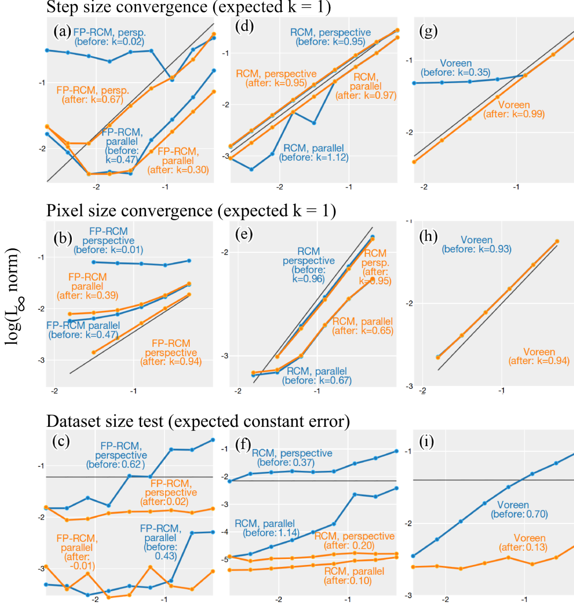
Figure 5.6. Each plot shows the convergence experiments for one particular implementation and one particular type of convergence. The behavior before any changes to the source code were made are shown in blue. The results of the changes are shown by the orange lines. The black line indicates the expected slope from the theoretical analysis. Notice the black lines indicate only the expected slope of the results. Any line parallel to the black indicator line has the same slope and is equally acceptable. The convergence order is denoted by k . Notice also that the dataset refinement test does not introduce errors and thus all that is expected is a constant error.
