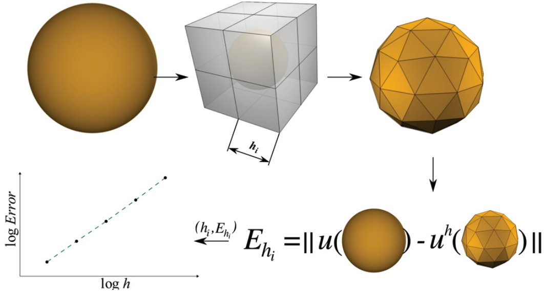
Figure 2.1. Workflow for the method of manufactured solution (Algorithm 1), clockwise from the top left.
