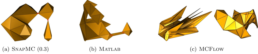
Figure 3.8. Mismatches in topology and geometry. (a) SNAPMC generates nonmanifold surfaces due to the snap process. (b) MATLAB generates some edges (red) that are shared by more than two face. (c) MCFLOWbefore (left) and after (right) fixing a bug that causes the code to produce the expected topology, but the wrong geometry.
