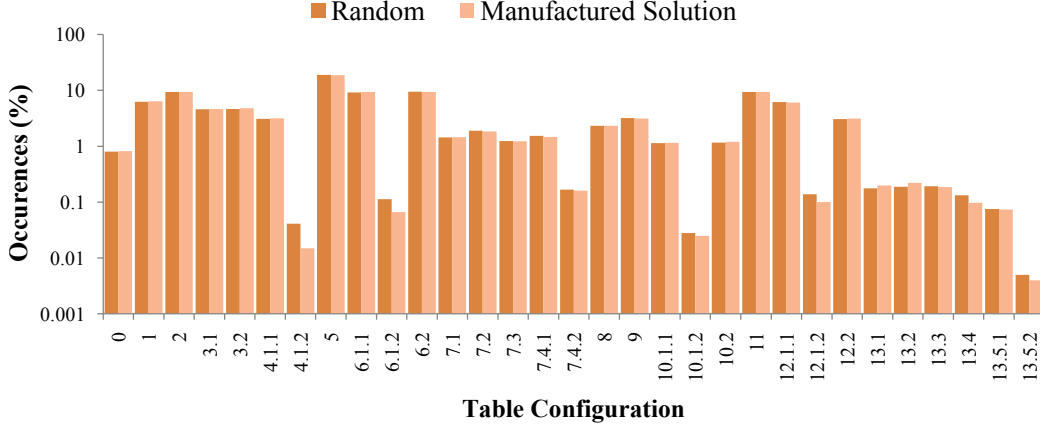
Figure 3.9. The horizontal axis shows the case and subcase numbers for each of the 31 Marching Cubes configurations. The dark bars show the percentage of random fields that fit a particular configuration. The light bars show the percentage of random fields that fit a particular configuration and do not violate the assumptions of our manufactured solution.
