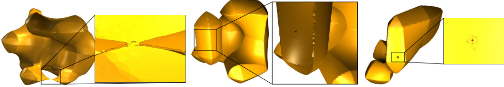
Figure 3.7. DELISO mismatch example. From left to right: holes in C^0 regions; single missing triangle in a smooth region; duplicated vertex (the mesh around the duplicated vertex is shown). These behaviors induce topology mismatches between the generated mesh and the expected topology.
