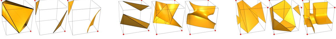
Figure 3.10. MC33 mismatch example. From left to right: problem in the case 4.1.2, 6.1.2, and 13.5.2 of Marching Cubes table (all are ambiguous). Each group of three pictures shows the obtained, expected, and implicit surfaces. Our verification procedure can detect the topological differences between the obtained and expected topologies, even for ambiguous cases.
