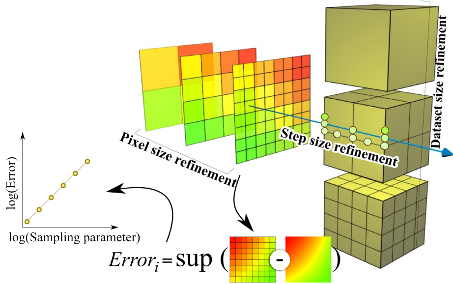
Figure 5.3. Our verification procedure works by evaluating discretization error during refinement of one of three sampling parameters.
