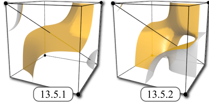
Figure 4.3. Challenging cases for Chernyave’s interior test: voxel diagonal has vertices with opposite signs. Case 13.5.2 needs to be oriented correctly. One of the diagonal vertices is isolated from all other vertices in the cube, while the other is faced by the tunnel. In order to determine which vertex is isolated, we apply the same tool used for disambiguation of case 13.5. For case 13.5.1, the orientation of the isosurface have no influence on the topology.
