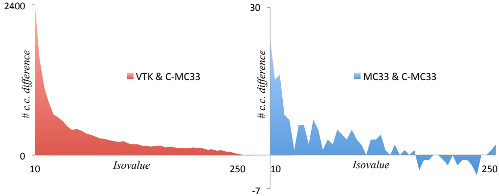
Figure 4.12. The left plot shows the difference between the number of connected components extracted by VTK implementation of Marching Cubes and the number of connected components extracted by our C-MC33 implementation. The right plot shows the difference in the number of connected components but between the MC33 and C-MC33 implementations. Negative values indicate that the C-MC33 implementation generated more connected components. Clearly, VTK generates more components than C-MC33. MC33 generates more components for most of the isovalue.
