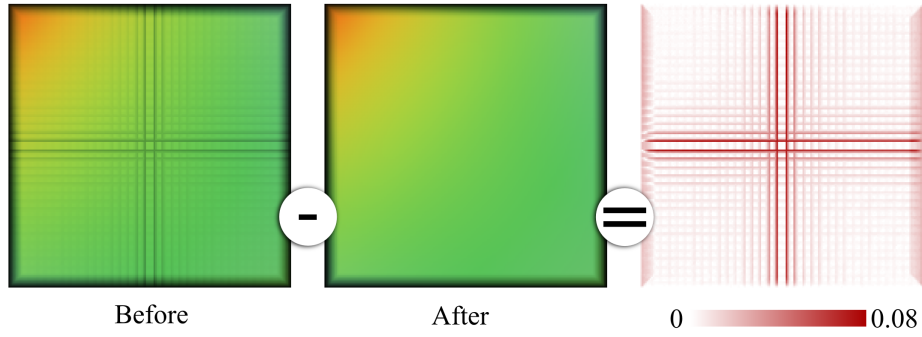
Figure 5.7. The figure shows images rendered using VTK 5.6.1. In our experiments, the ‘+’ pattern became more evident in two cases: when coarse datasets are used, and/or high number of sampling points along the ray are used. Darker pixels belong to regions where the ray traverses only half of the volume, preventing convergence. The image on the middle shows the result using our modified version of VTK. The convergence curve improved significantly after the issue was fixed. Note that this effect only occurs when perspective projection is used. For orthogonal projection, the problem is not noticeable. For the convergence analysis, we used a scalar field given by S(x, y, z) = xyz , D = 1 , transfer function \tau(s) = s in the domain [0, 1]^3 , and solution for the VRI given by I(x, y) = 1 - \exp(-xy/2) , which means the integration is along z (from zero to one).
