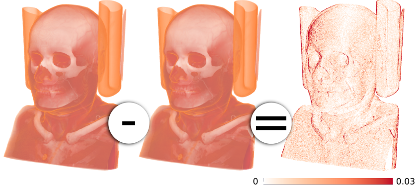
Figure 5.2. Expert analysis and error quantification may fail to detect problems. Left: the volume rendering of the torso dataset using an incorrect trilinear interpolation. Middle: same dataset with the correct interpolation. Right: difference between the two images.
