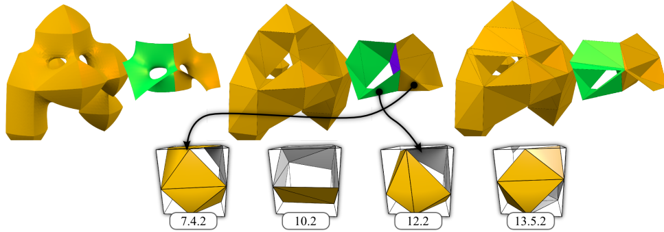
Figure 4.7. Top: Problem with Chernyaev’s triangulation table. The figure shows the zero level-set of a 5 \times 5 \times 5 randomly generated piecewise-trilinear scalar field G (left) and two meshes extracted using the MC33 (center) and C-MC33 (right) algorithms. The isolated voxel patches, shown in green and yellow, represent the two voxels at the center of G . The face shared by two consecutive tunnels, shown in purple, generates nonmanifold edges. After one subdivision at the critical point of this case, the problem no longer occurs, and a valid manifold surface is obtained (right). Bottom: Triangulation for tunnels used by Lewiner et al. [94]. Each has a face that is coplanar to the voxel faces, which may lead to nonmanifold surfaces [28].
