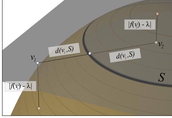
Figure 2.2. The distance between a point \vec{v} and the isosurface S with isovalue \lambda can be approximated by the algebraic distance divided by the gradient magnitude of the scalar field at \vec{v} , |f(\vec{v}) - \lambda|/|\nabla f(\vec{v})| . In the figure, the thick circle represents the isosurface S and the fainter isolines illustrate changes in gradient magnitude: in regions of small gradient magnitude, the algebraic distance is small but geometric distance is large, and vice-versa for large gradient magnitude.
