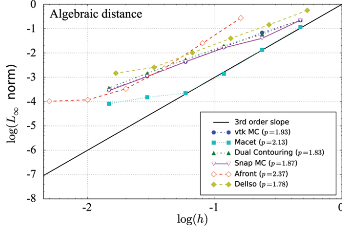
Figure 2.7. Order of accuracy for a transcendental function f(x, y, z) = x^2 + y^2 + z^2 + \cos(Ax)^2 + \cos(Ay)^2 + \cos(Az)^2 , A is a constant. The observed orders of accuracy for all implementations are relative to the voxel size h . We expect third-order accuracy for Afront and Macet due to their use of high-order spline approximations. Both have the expected convergence rate for all but the last two values.
