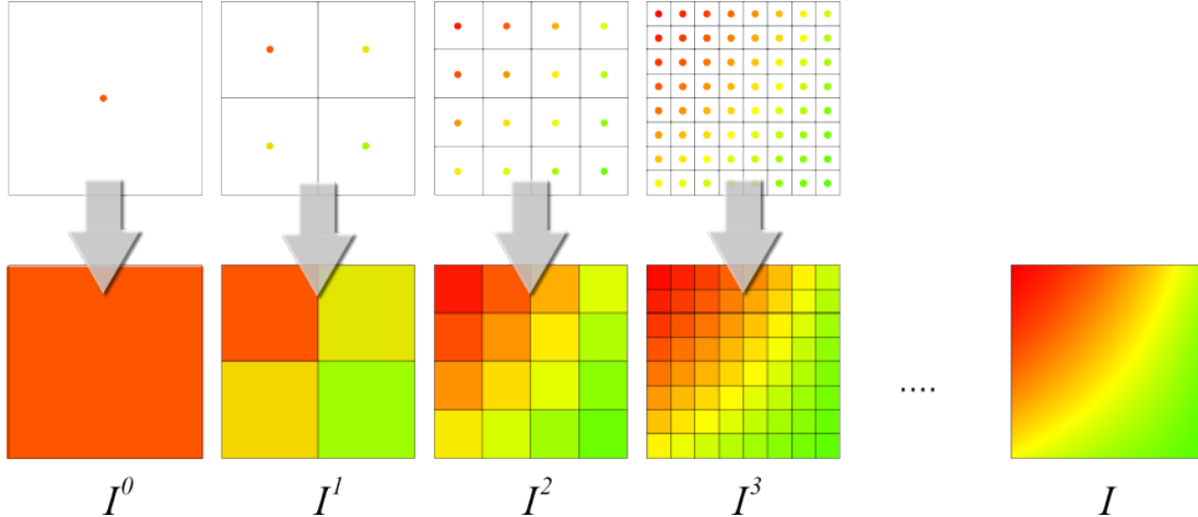
Figure 5.5. Pixel refinement. Typically, the VRI is evaluated only at pixel centers (top). The value at the center is then interpolated in the domain defined by the pixel size (bottom) using nearest-neighbor interpolation to obtain \tilde{I}^i . In a correct implementation, as i increases, \tilde{I}^i approaches the true solution I .
