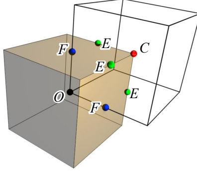
Figure 3.3. The four distinct groups of vertices O, F, E, C , are depicted as black, blue, green, and red points. They are the “Old”, “Face”, “Edge,” and “Corner” points of a voxel region V_G (semitransparent cube), respectively. For the sake of clarity, we only show a few points.
