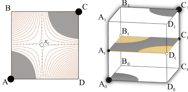
Figure 4.2. Asymptotic Decider (left) and MC33 interior ambiguity test for MC case 4 (right). The gray areas represent regions with positive scalar values, and the capital letters represent the scalar value at each vertex. In the left image, we observe that f(x_c) < 0 , where x_c is the saddle point position. Positive areas will be connected if f(x_c) > 0 . The orange squared plane shown in the right image represents the cutting-plane. The goal of the MC33 algorithm is to find a cutting-plane such that the gray areas in the top and bottom planes are joined in the interior.
