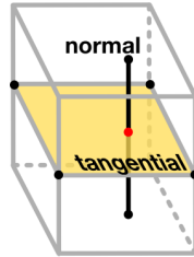
Figure 3.5. Example of tangential and normal link.
