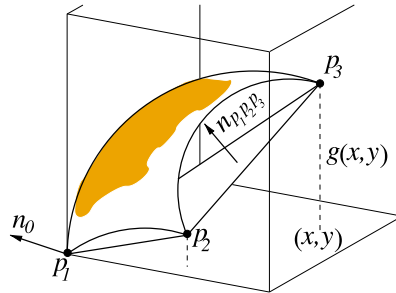
Figure 2.3. Isosurface local parametrization and approximation.
