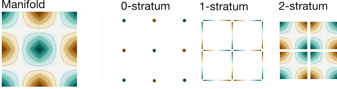
Figure 3.4. An illustration of a piecewise-smooth immersed 2-manifold. The colormap illustrates the value of each point of the scalar field. Notice that although the manifold itself is not everywhere differentiable, each stratum is itself an open manifold that is differentiable.
