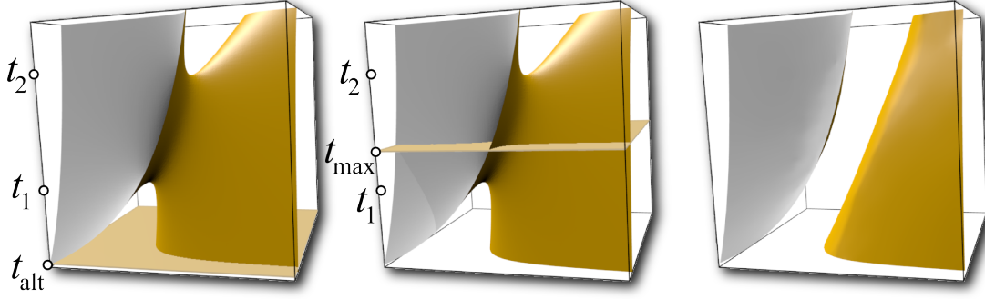
Figure 4.8. Case 6 configuration. Left: the cut plane height t = t_{\text{alt}} > 0 used in the MC33 implementation . Middle: the test proposed in the MC33 algorithm provides a different t = t_{\text{max}} > 0 , which reaches the tunnel. Right: the former test decides that the isosurface is homeomorphic to two discs whereas the correct answer is a tunnel [28].
