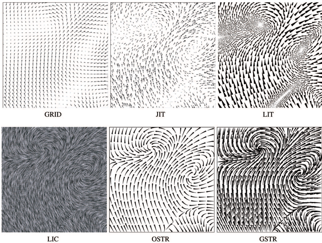
Figure 6.5. Comparing visualization methods for steady 2D vector fields [86]. Top: standard arrow visualization, jittered arrow, icons using concepts borrowed from oil painting, respectively. Bottom: line-integral convolution, image-guided streamlines, streamlines seeded in a regular grid, respectively. Image used with permission.
